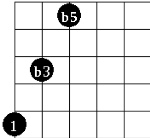
Root Position
