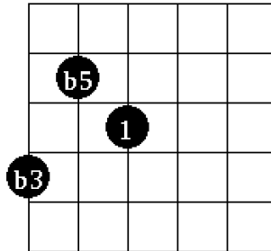
1st Inversion
