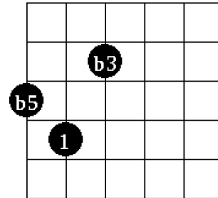
2nd Inversion
